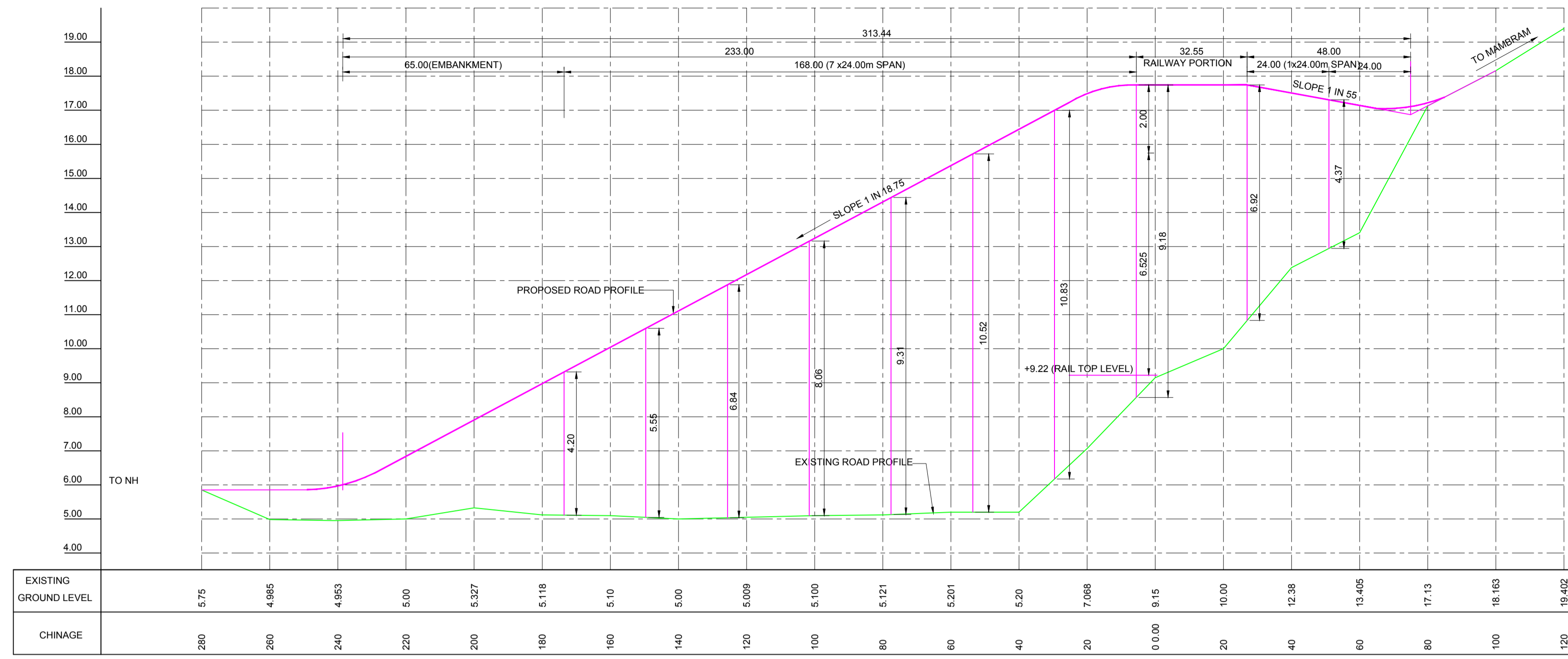
LONGITUDINAL PROFILE SCALE HOR: 1:1000 VER: 1:100
